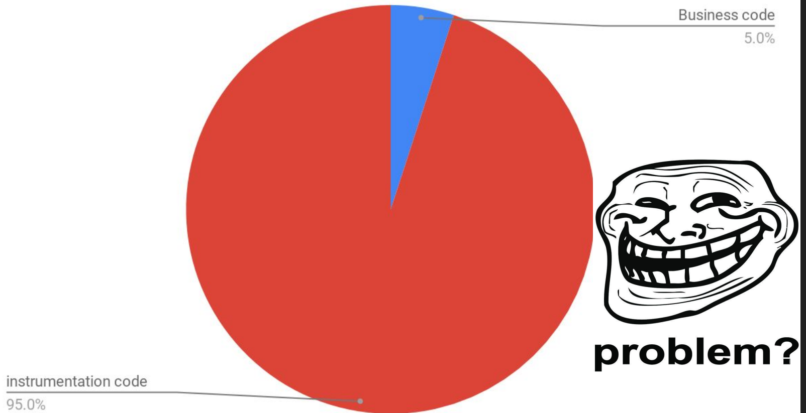
Code distribution
